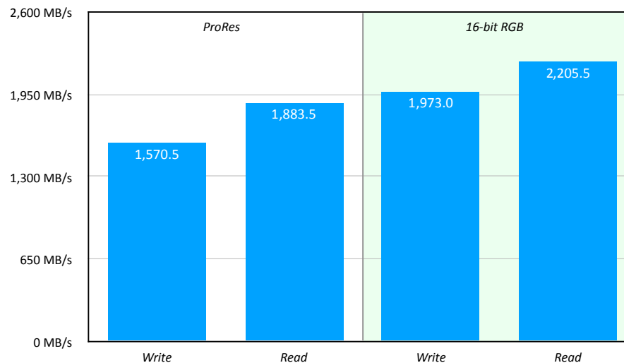
1920 x 1080 ProRes vs. 16-bit RGB Tests
