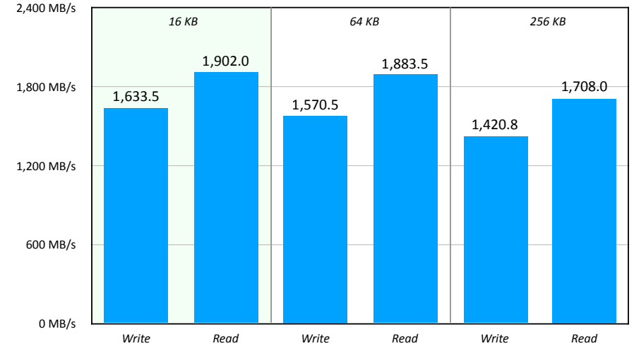
1920 x 1080 ProRes Speed Tests by RAID Chunk Size
